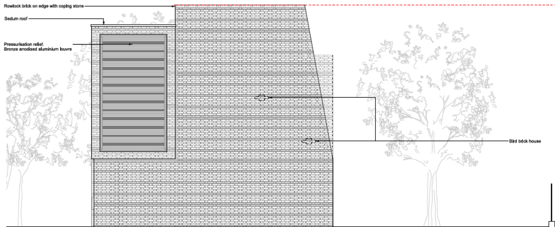
01 GENERAL ARRANGEMENT - EAST ELEVATION
