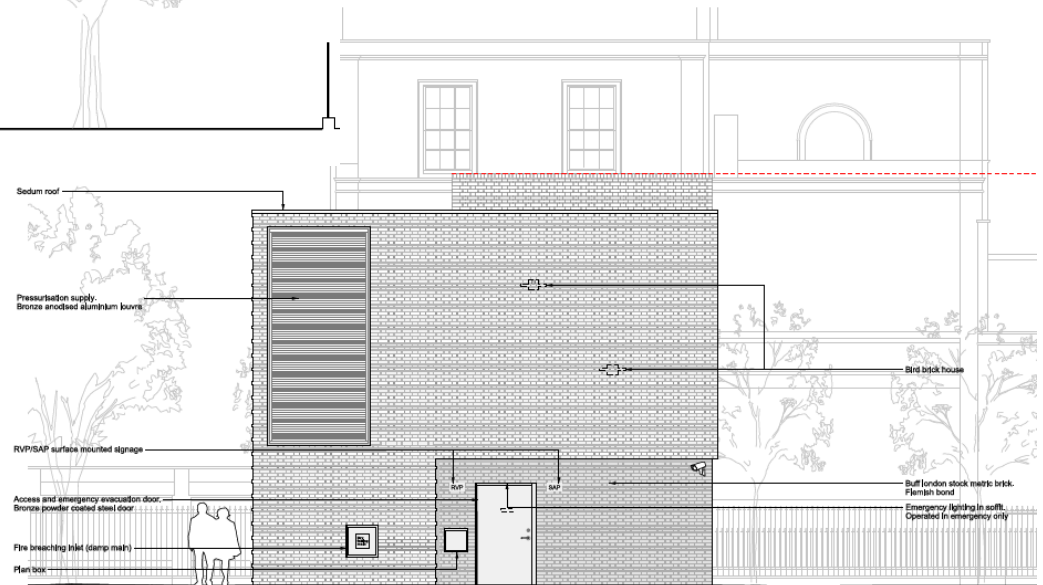
02 GENERAL ARRANGEMENT - SOUTH ELEVATION
