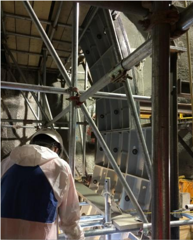
Installation of SGI rings W/C – 09/01/2017
