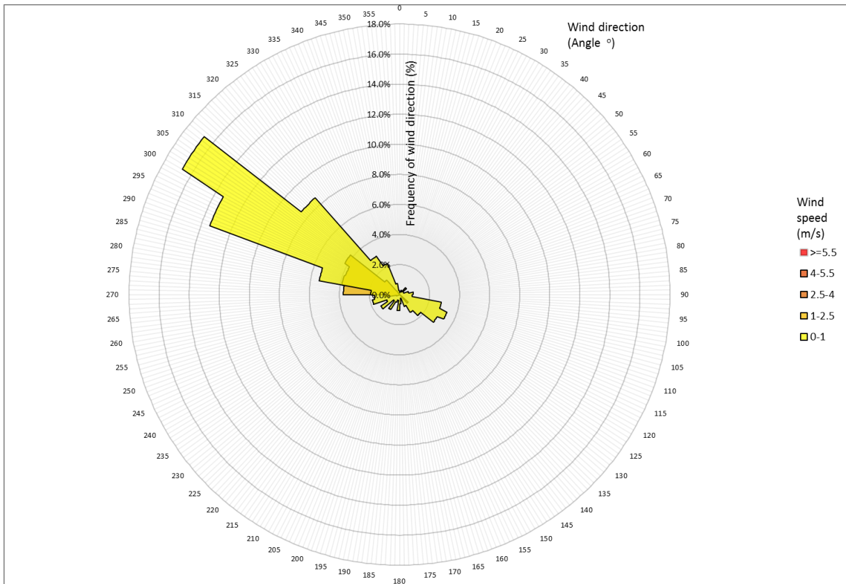
Figure 2. Wind rose from the Kennington Green sonic anemometer KG1W. Period 2.
