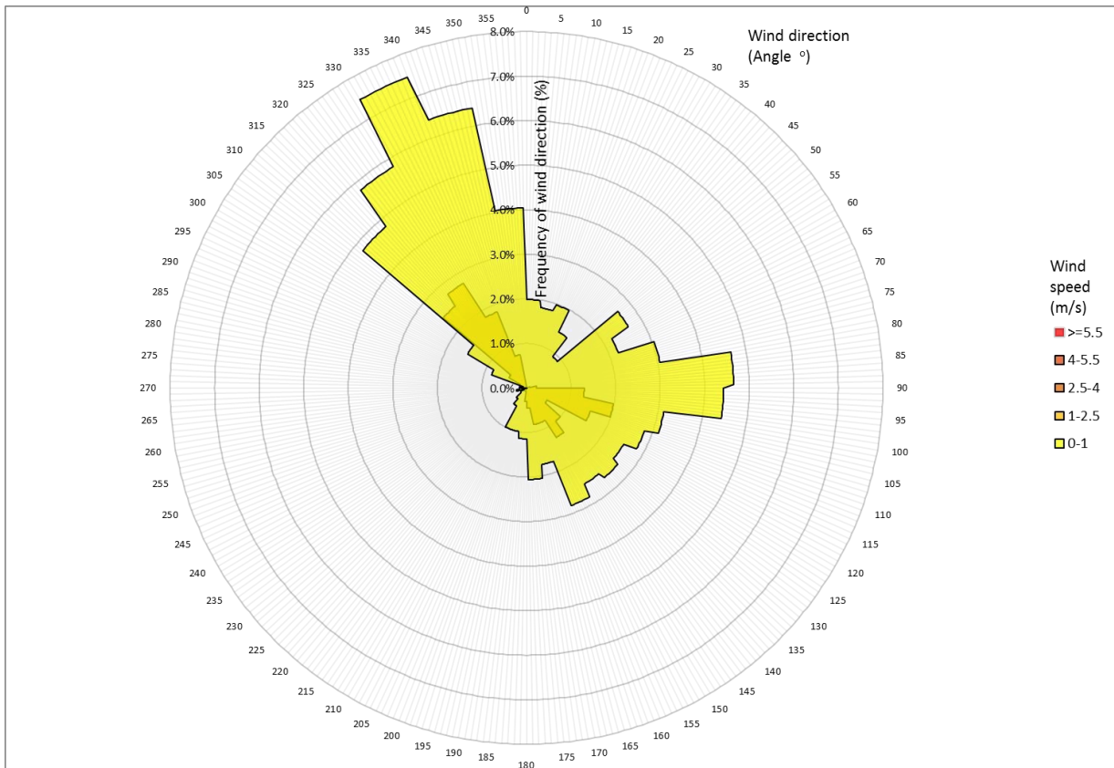
Figure 2. Wind rose from the Nine Elms sonic anemometer NE2_2094 W, period 2.
