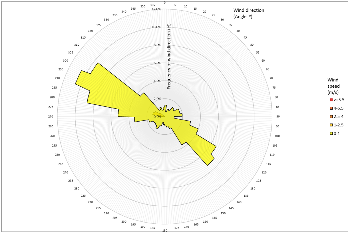
Figure 3. Wind rose from the Kennington Park sonic anemometer KP2W. Period 3.
