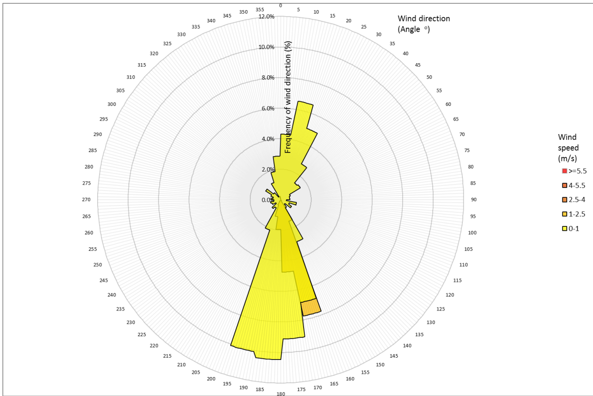
Figure 3. Wind rose from the Kennington Green sonic anemometer KG1W. Period 3.
