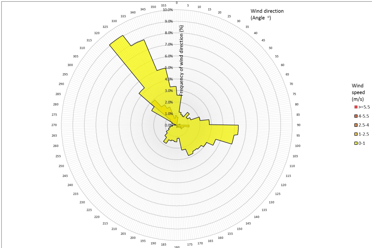
Figure 2. Wind rose from the Battersea sonic anemometer BAW3 Period 2.
