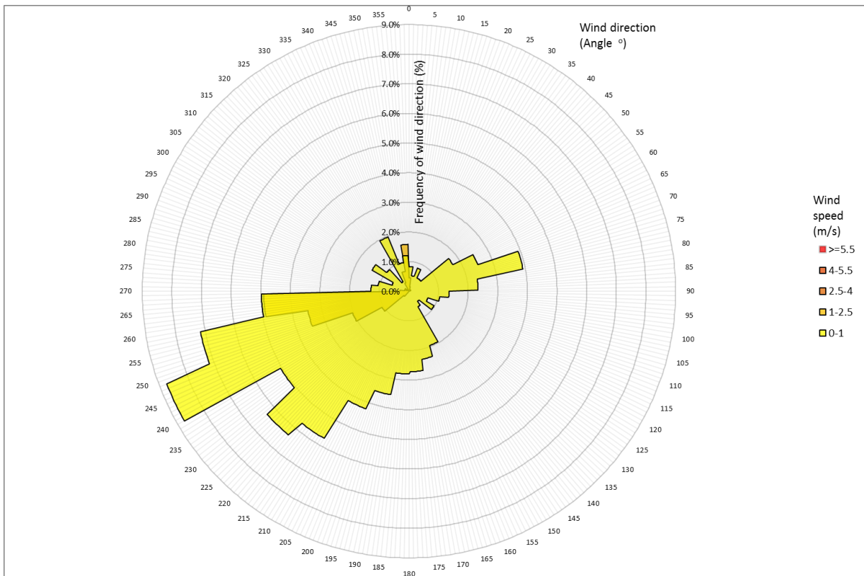
Figure 3. Wind rose from the Battersea sonic anemometer BN2W. Period 3.
