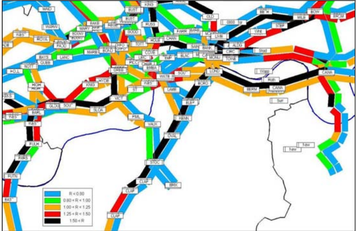
Figure 14 Underground Crowding Ratios, 2008 Morning Peak Period (7-10am)
