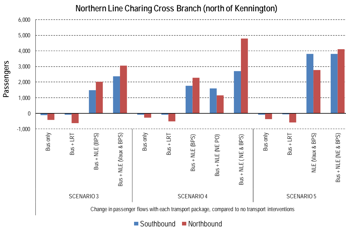
Figure 51 Change in Northern Line (Charing Cross) Passenger Flows, 2026 Morning Peak Period (7-10am)
