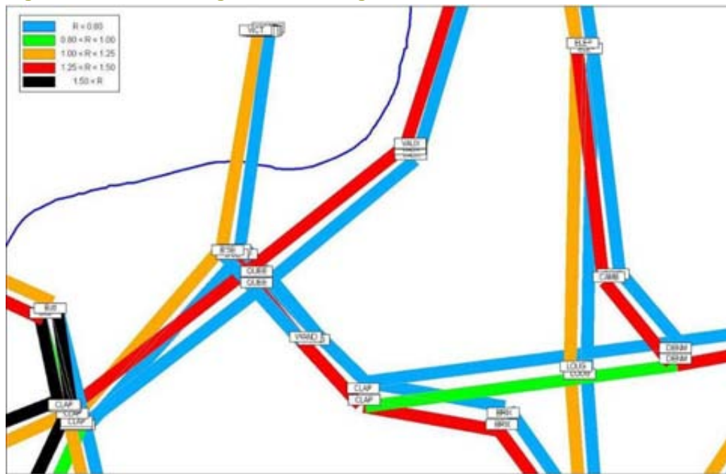
Figure 36 Rail Morning Peak Crowding Ratios, 2026 Reference Case
