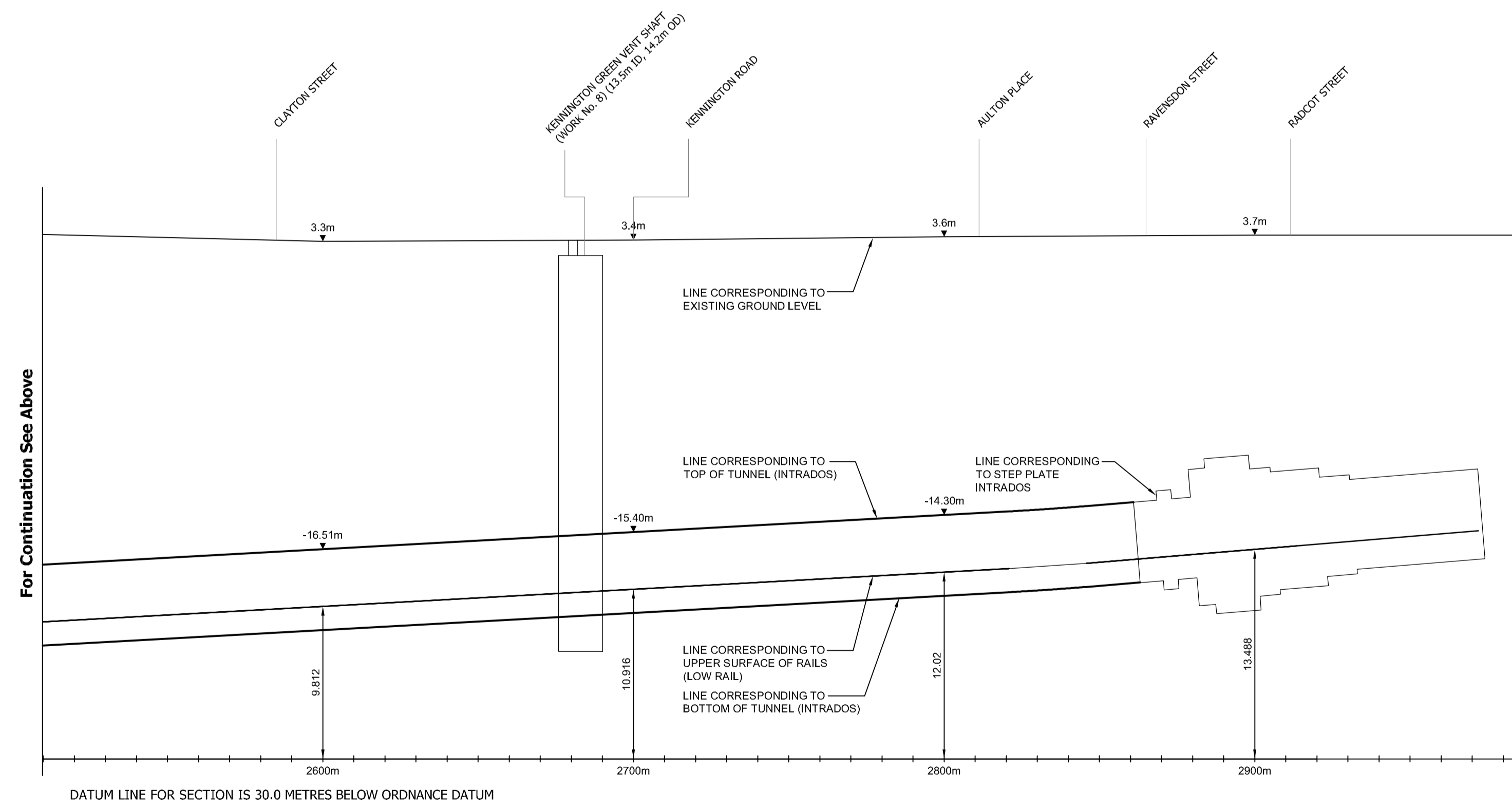
NORTHBOUND WORK No.2
